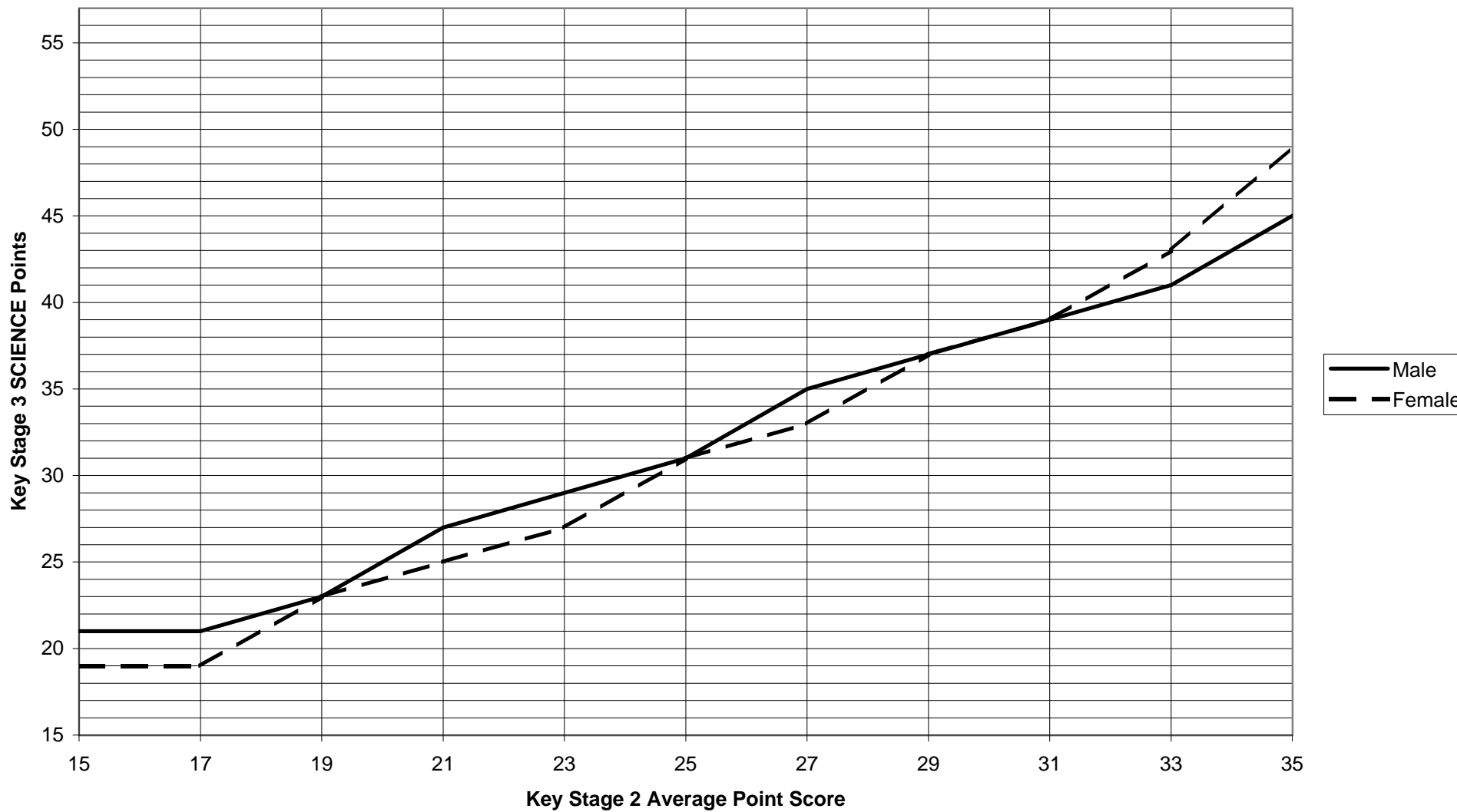
Hertfordshire Key Stage 3 2000 Science Median Lines by Gender
